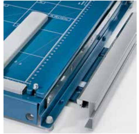
Pull-out front stop up to 170 mm with fold-out paper holders for cutting strips of equal width
